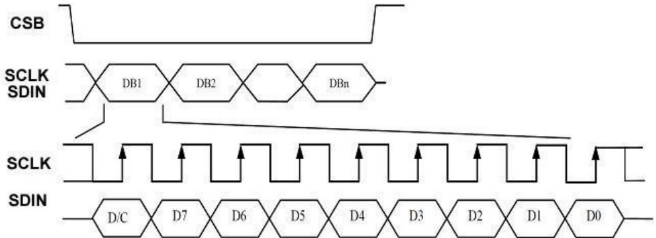
Write procedure in 3-wire SPI mode
